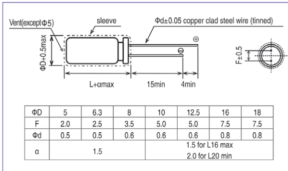
Outline Drawing
