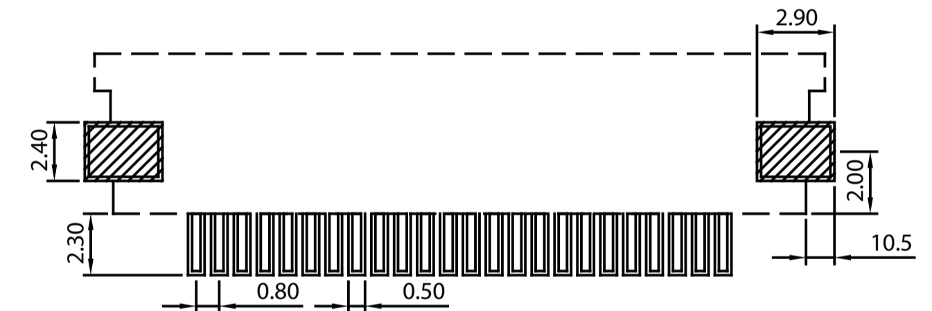
Recommended PCB Layout (PCB TOLERANCE ±0.05)
