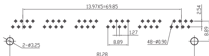
PC Board Layout
