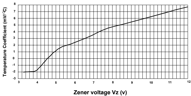
Temperature Coefficient
