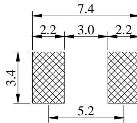
( PCB Pattern )
