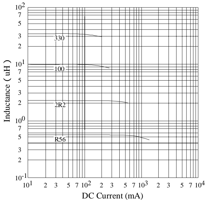
@ Inductance vs. DC Currnt curve.
