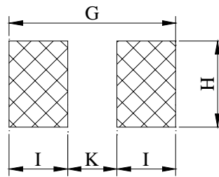
( PCB Pattern )
