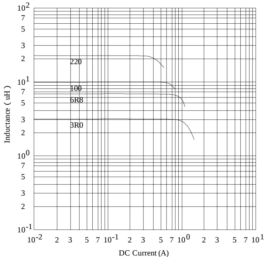
@ Inductance VS. DC Current Curve
