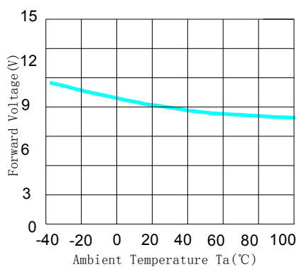
Fig.3 Forward Voltage Vs Ambient Temperature
