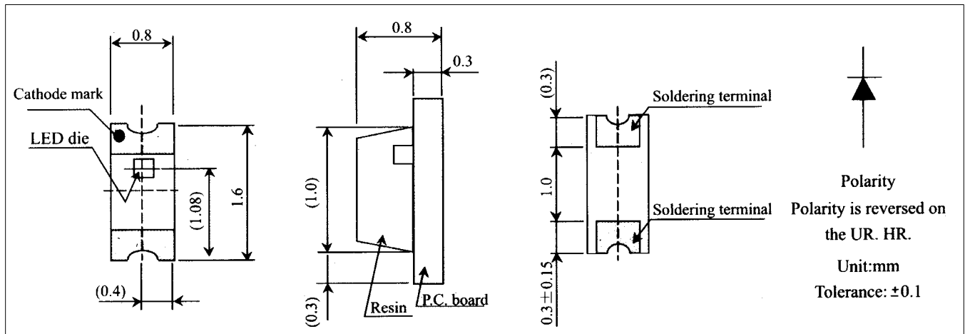
Dimensions: 1.6 (L) x 0.8 (W) x 0.8 (H) mm
