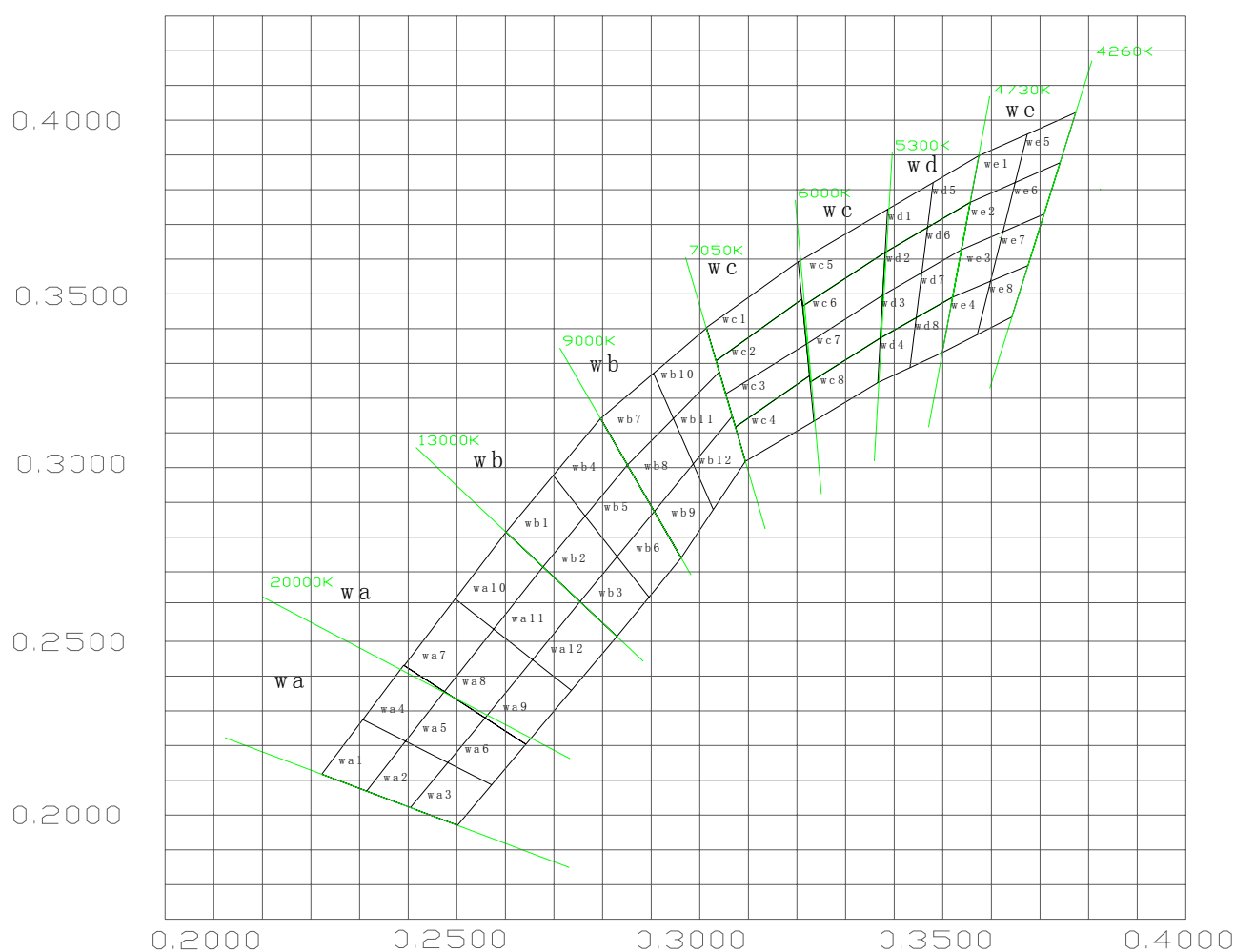
CIE 1931 Chromaticity diagram/CIE1931 图 (IF=30mA Ta=25℃)
