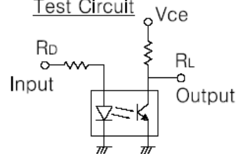
Test Circuit
