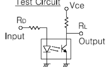
Test Circuit
