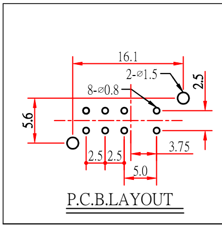
* CRITICAL DIMENSION
