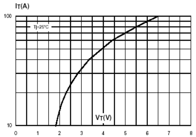
Fig. 2: On-state voltage versus on-state current (typical values)
