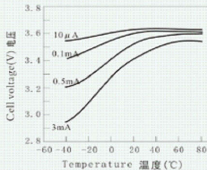
Voltage vs temperature 电压VS温度
