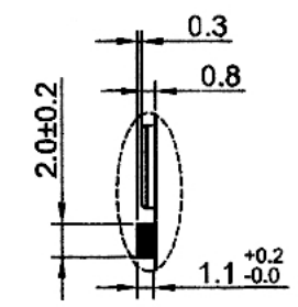
POLARITY PROTECTION DEVICE DETAIL "A" S=2
