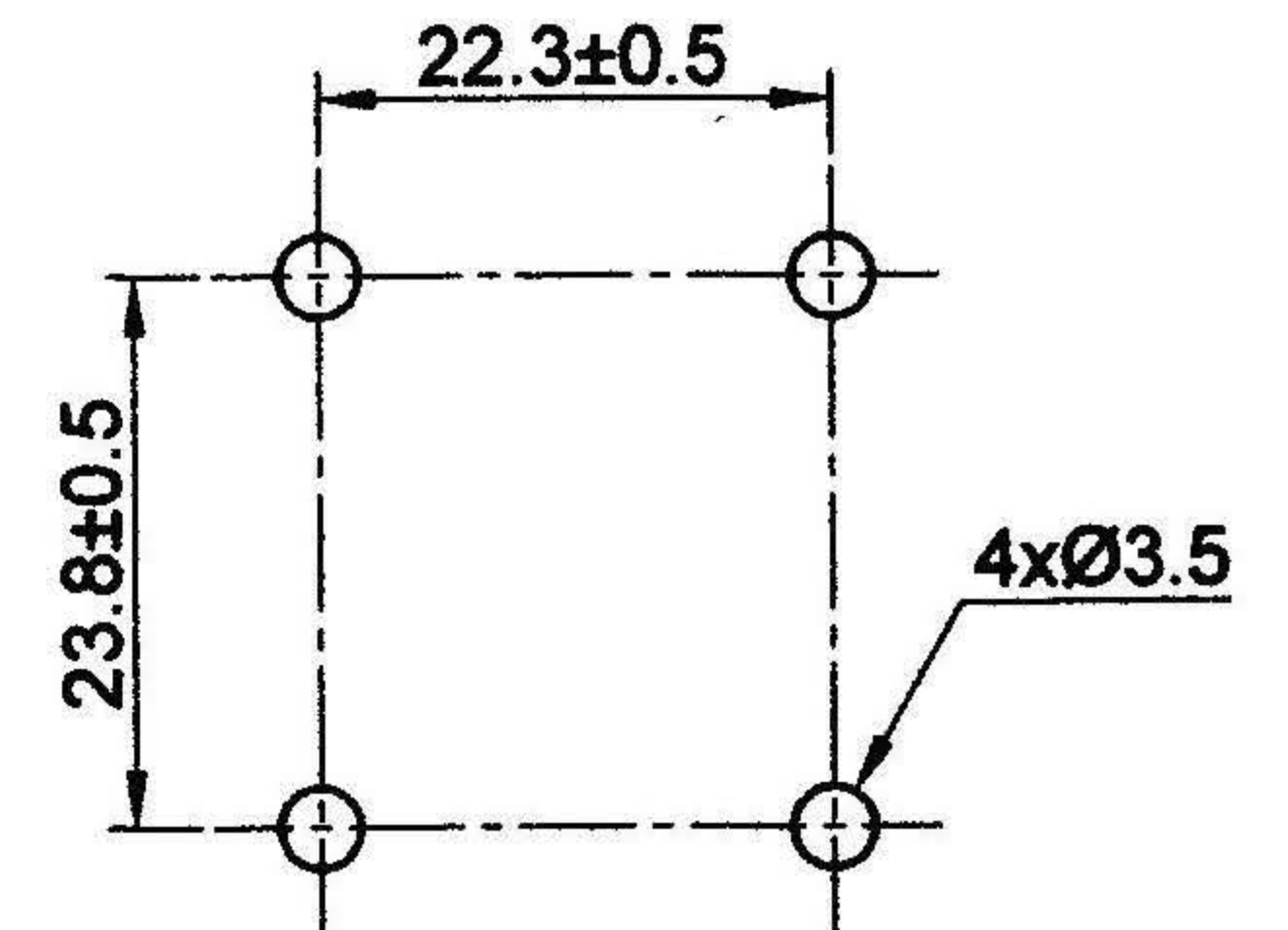
PCB/MOUNTING LAYOUT
