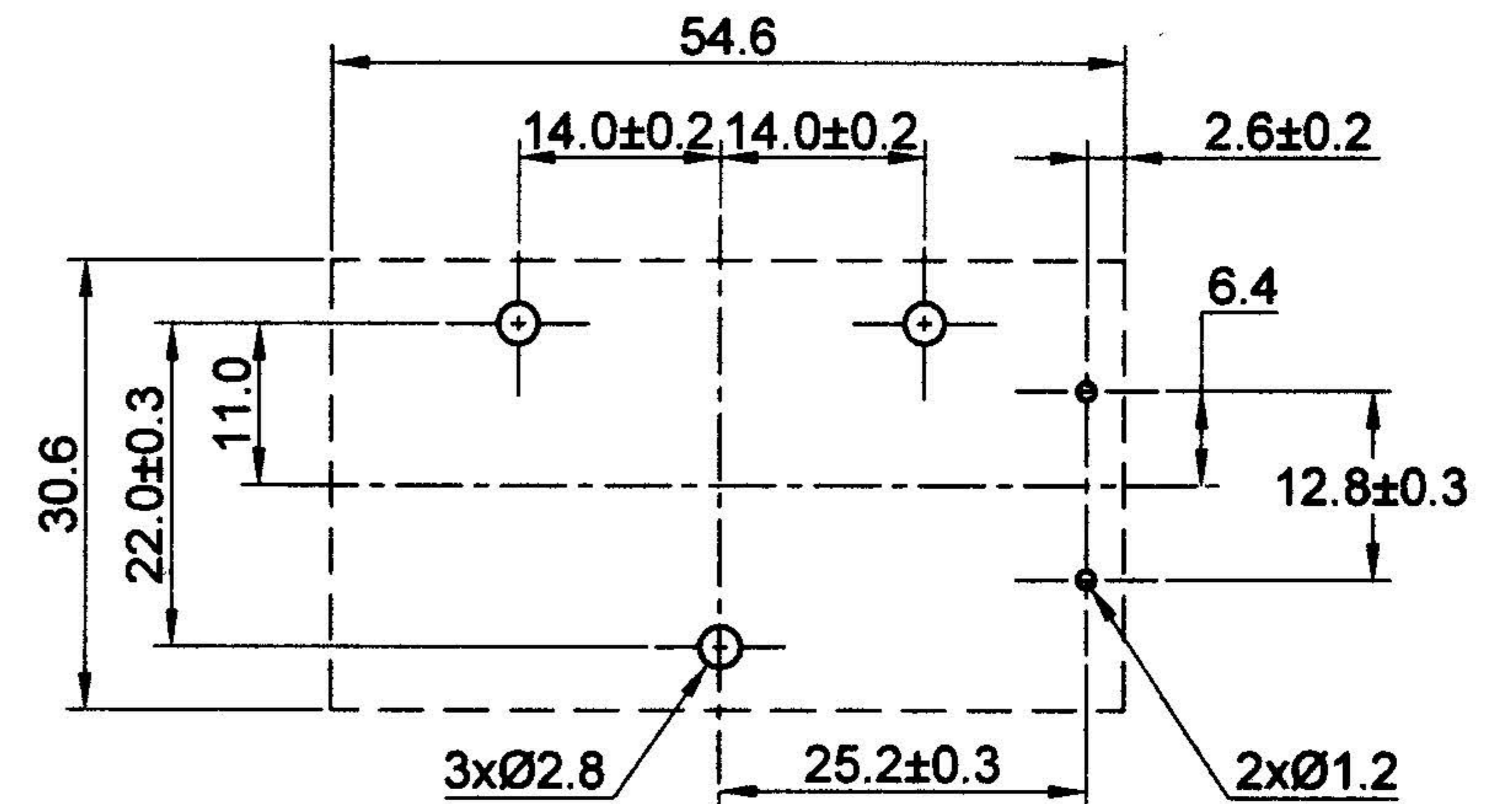
PCB/MOUNTING LAYOUT
