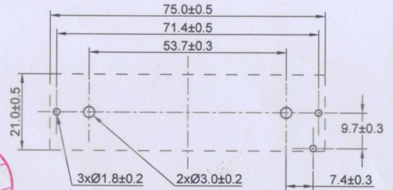
PCB/MOUNTING LAYOUT
