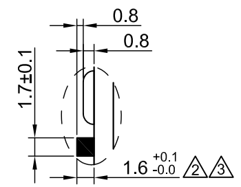
POLARITY PROTECTION DEVICE DETAIL "A" S=2
