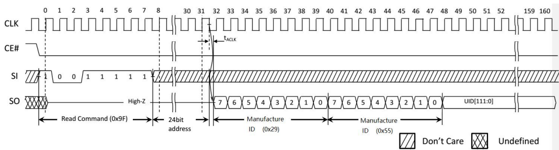
SPI Unique ID Register read 0x9F
