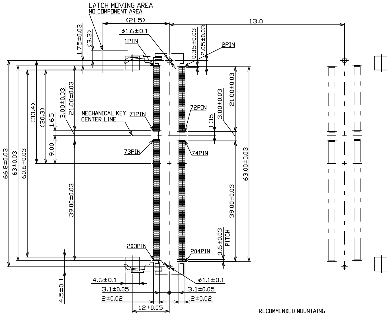
RECOMMENDED MOUNTING P.C. BOARD PATTERN LAYOUT DIM.
