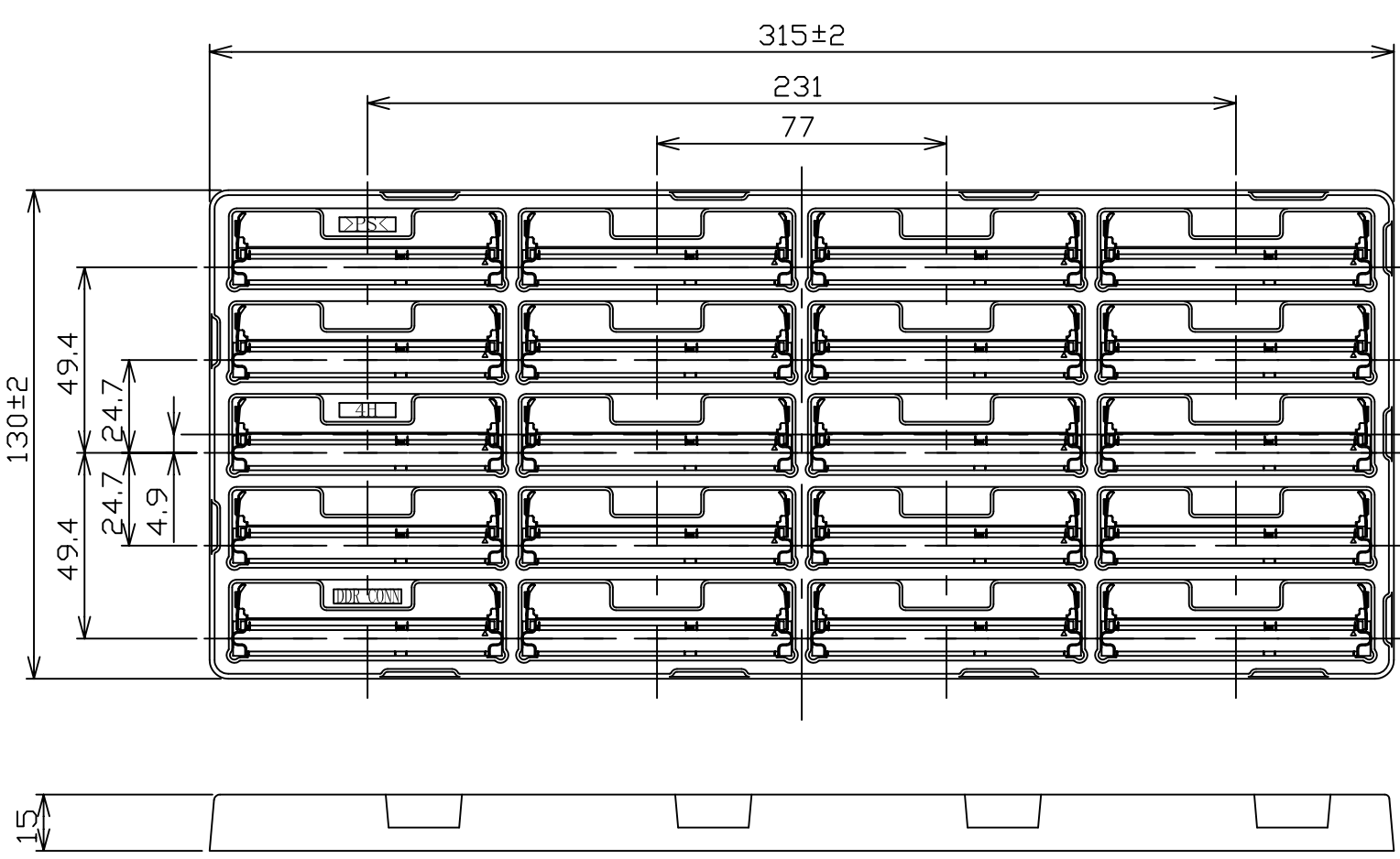
SOFT TRAY PACKAGING
