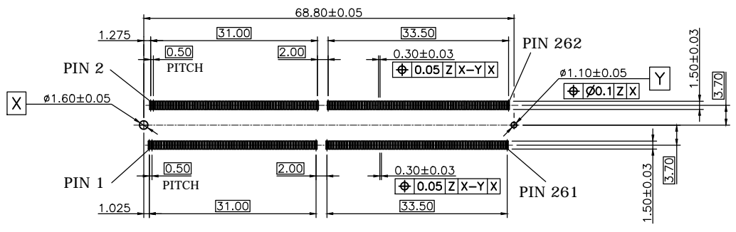
RECOMMENDED PCB LAYOUT (TOP VIEW) GENERAL TOLERANCE: ±0.05mm
