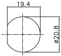
Panel Cut-Out
