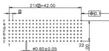
RECOMMENDED PCB-HOLE LAYOUT COMPONENT SIDE SHOWN
