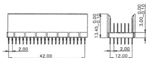
CONNECTOR ASSEMBLY EXEMPLARY LOADED
