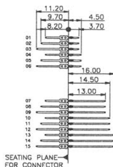
CONTACT DIMENSIONS
