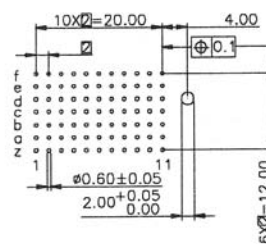
RECOMMENDED PCB-HOLE LAYOUT COMPONENT SIDE SHOWN
