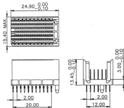
CONNECTOR ASSEMBLY EXEMPLARY LOADED
