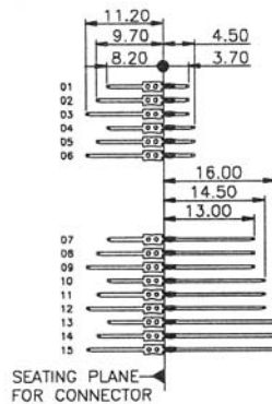
CONTACT DIMENSIONS
