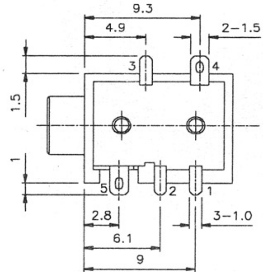
<BOTTOM VIEW>
