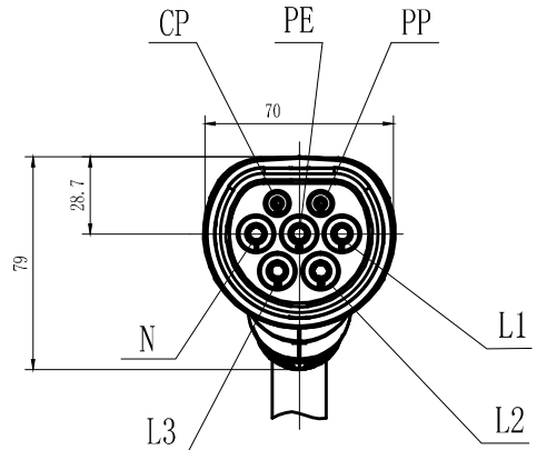
Wiring diagram
