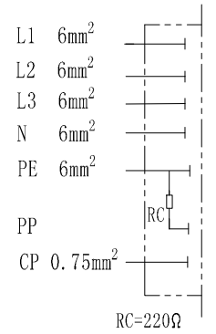
Wiring diagram
