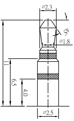
MATE PLUG
