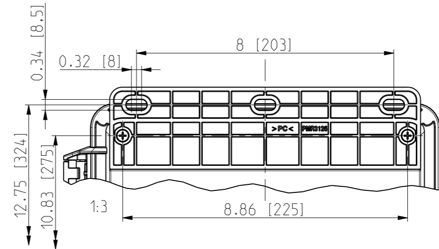
FRONT VIEW WITH COVER REMOVED
