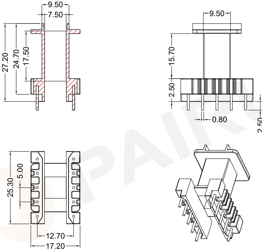
Winding data and area product for 10-pins EF25/13/7 coil former
