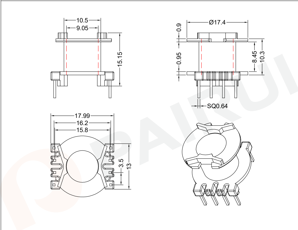
Winding data and area product for 8-pins PQ20/16 coil former
