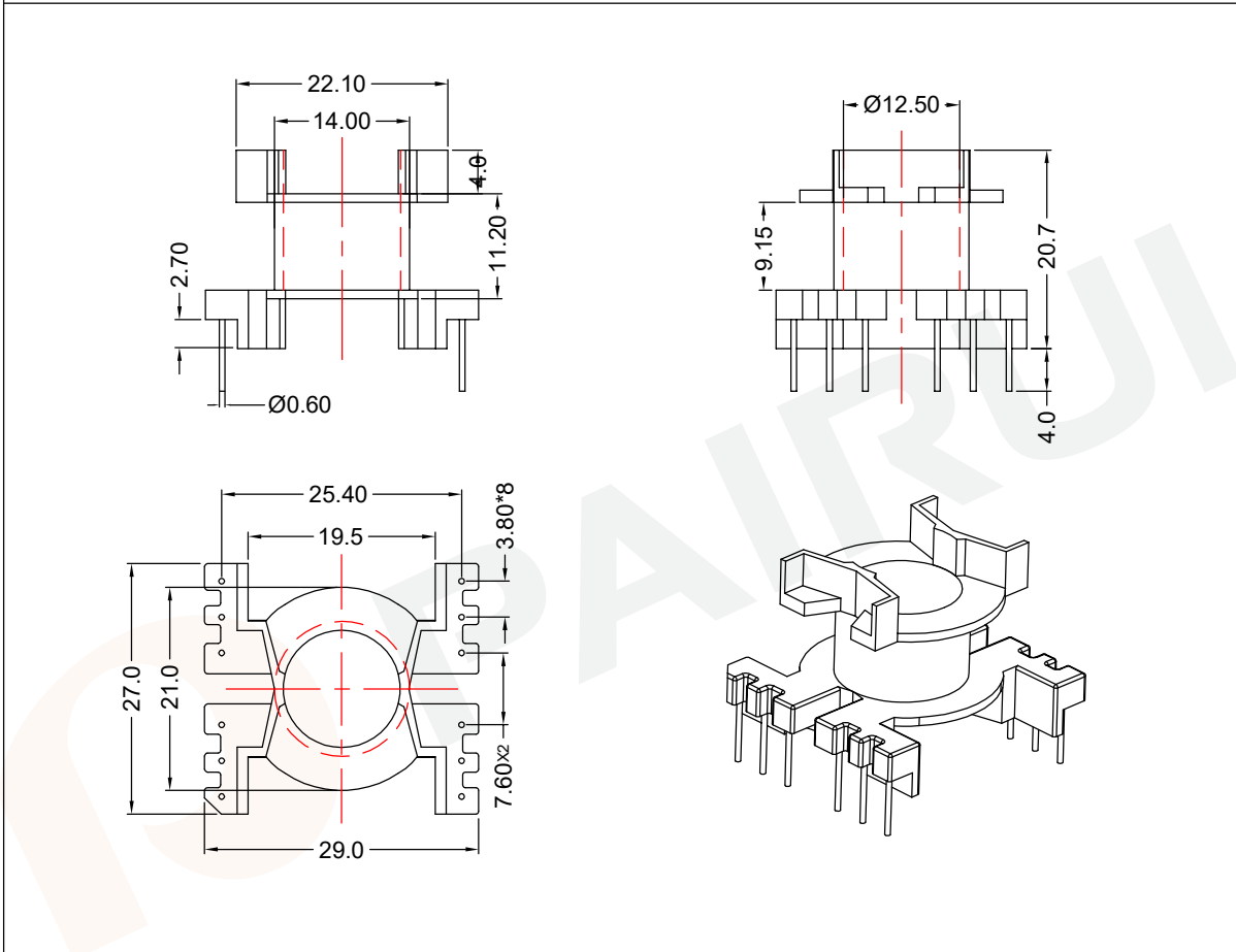
Winding data and area product for 12-pins PQ26/20 coil former
