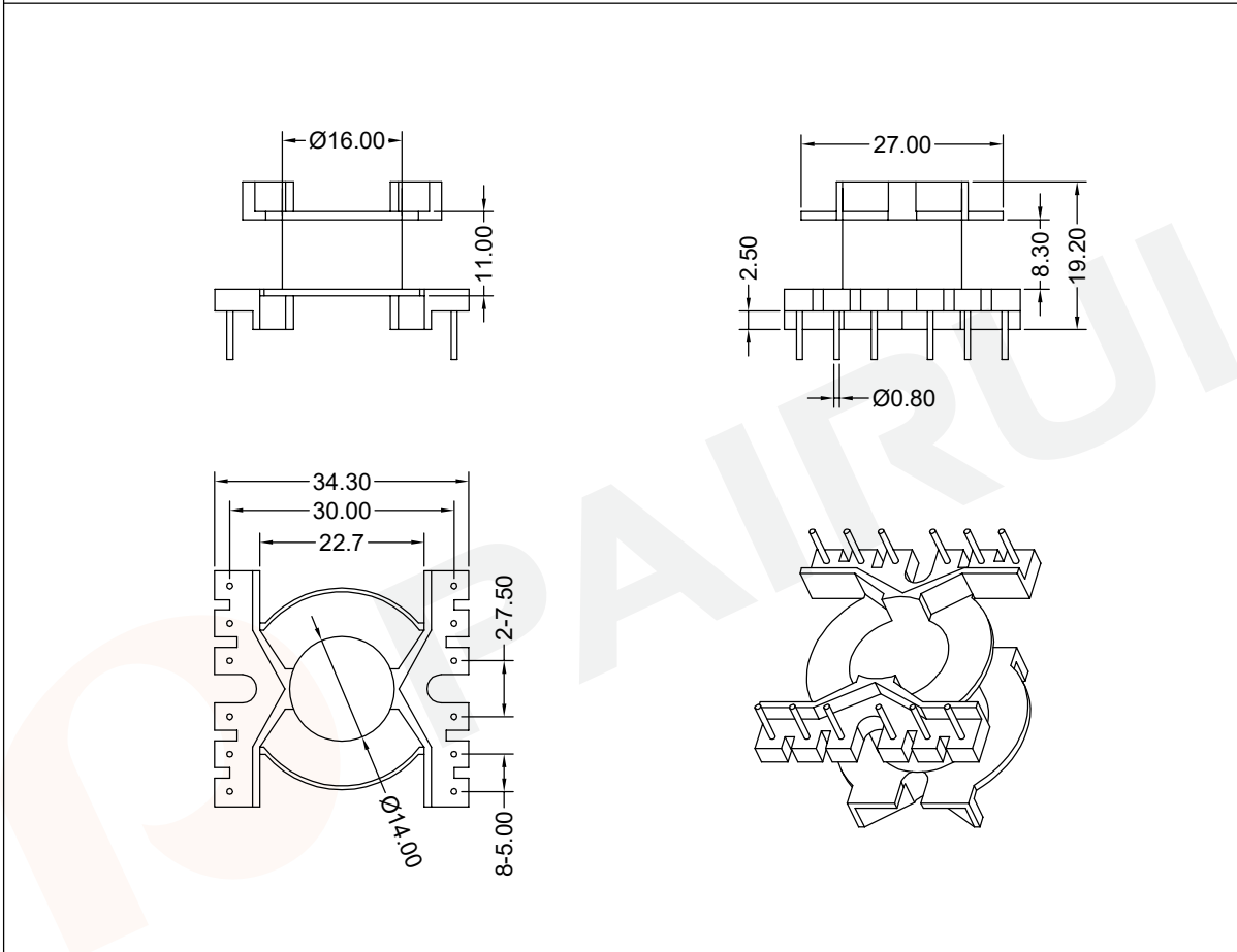
Winding data and area product for 12-pins PQ32/18 coil former
