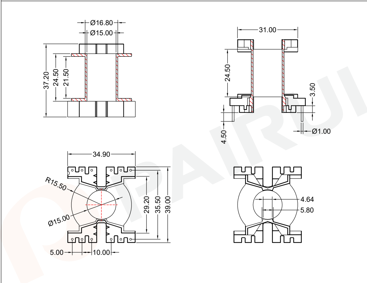
Winding data and area product for 12-pins PQ35/35 coil former
