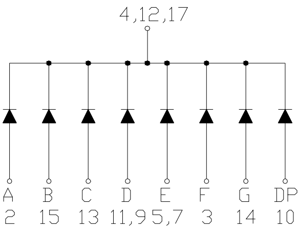
No.:1,6,8,16,18 NO Pin Common Cathode
