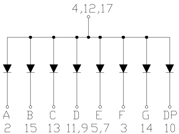
No.:1,6,8,16,18 NO Pin Common Anode
