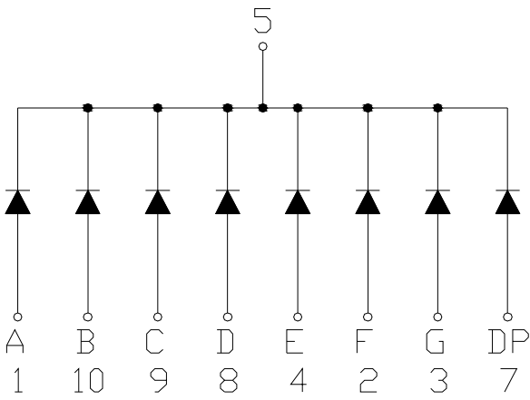
No.: 6,11,12 NO Pin Common Cathode
