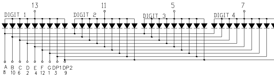
Common Anode
