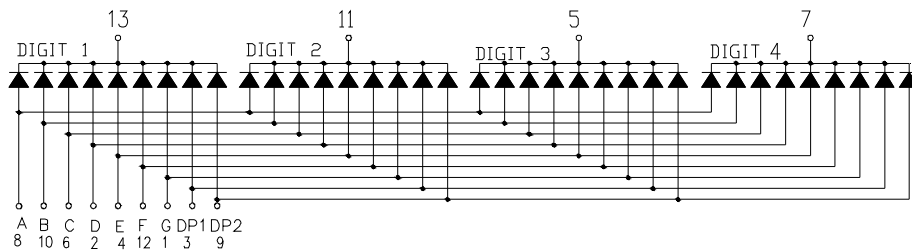
Common Cathode
