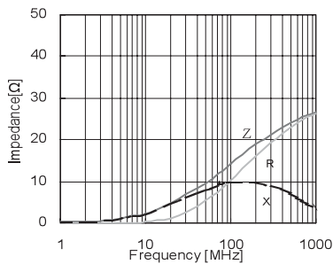
CBW160808U190T
