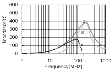
CBW321609U301T
