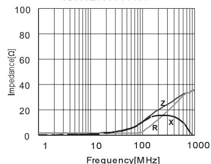
CBW321609U110T
