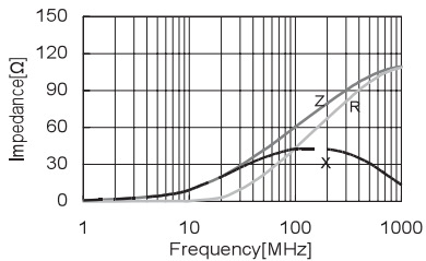
CBW321609U600T
