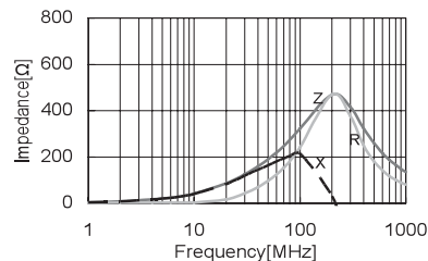
CBW201209U301T
