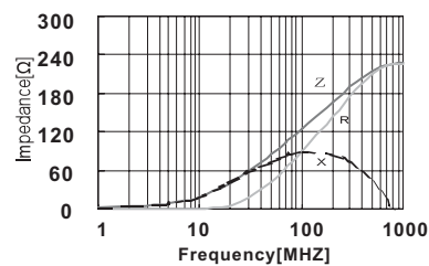
CBW453215U121T
