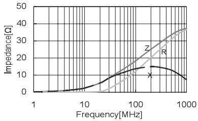
CBW321609U190T
