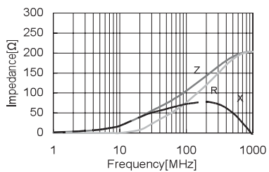
CBW453215U101T
