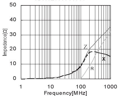
CBW321609U090T
