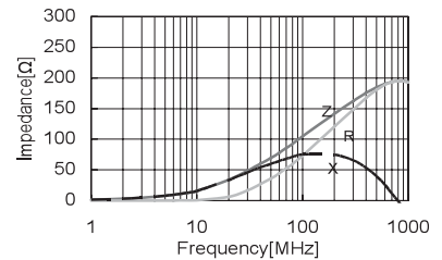
CBW321609U101T
