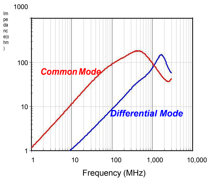
IMPEDANCE vs. FREQUENCY CHARACTERISTICS
