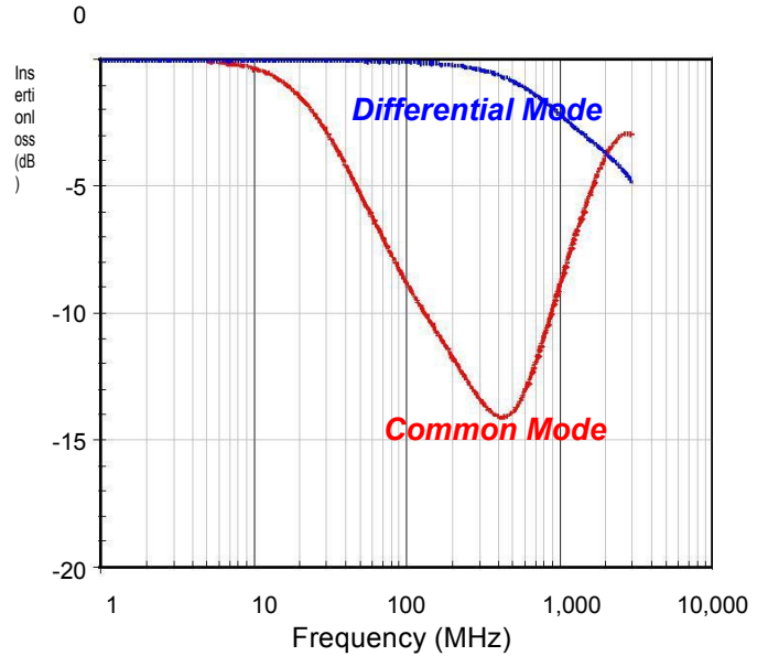
INSERTION LOSS vs. FREQUENCY CHARACTERISTICS
