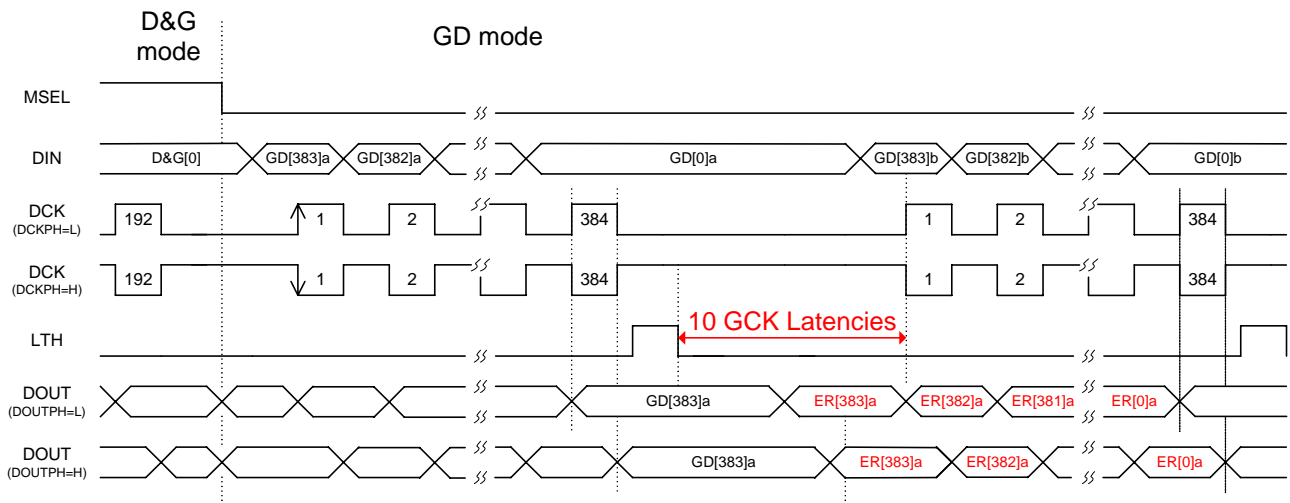
Figure 4. GD Mode Data Input Timing Chart
