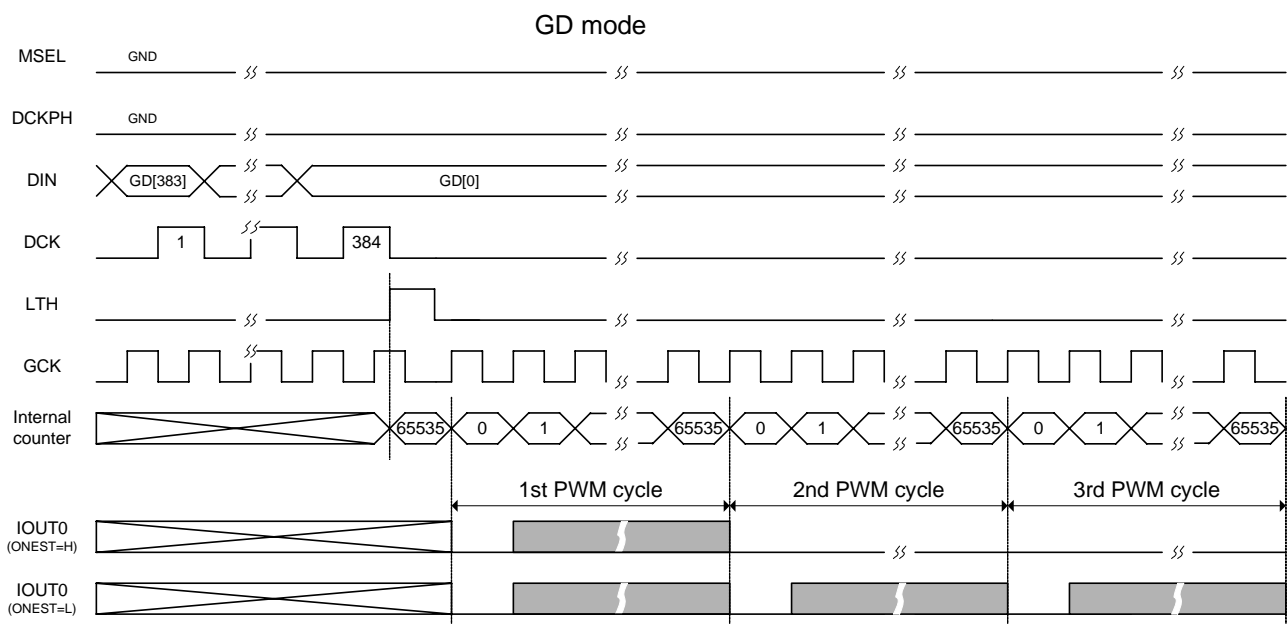
Figure 9. One-Shot Operation
