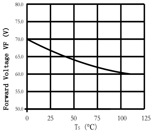
Case Temperature vs. Forward Voltage 结点温度与正向电压曲线图 I_F=1300\text{mA}
