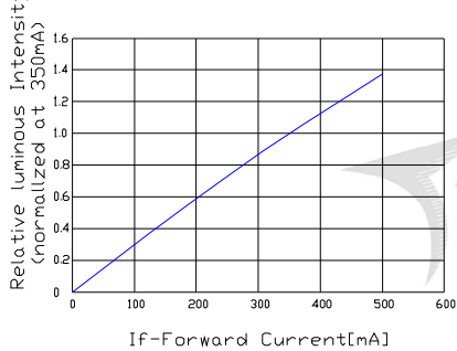
Fig.1-Relative luminous Intensity vs. Forward Current
