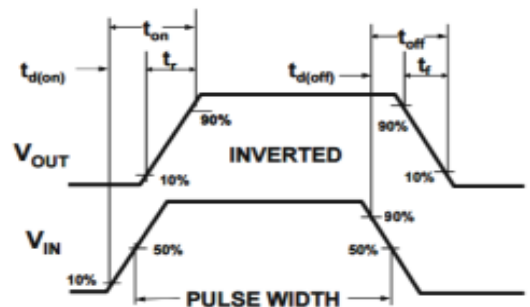
Figure8. Switching wave
