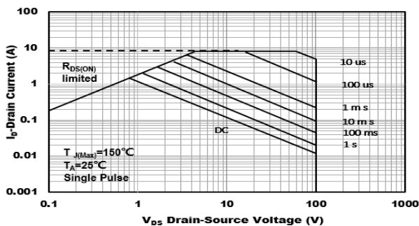
Figure7. Safe Operation Area
