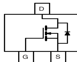
SOT-23 (Marking: S2)
