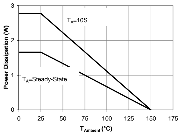
Figure 12: Power De-rating
