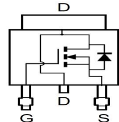
TO-252
