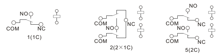
Wiring diagram (Bottom views)
