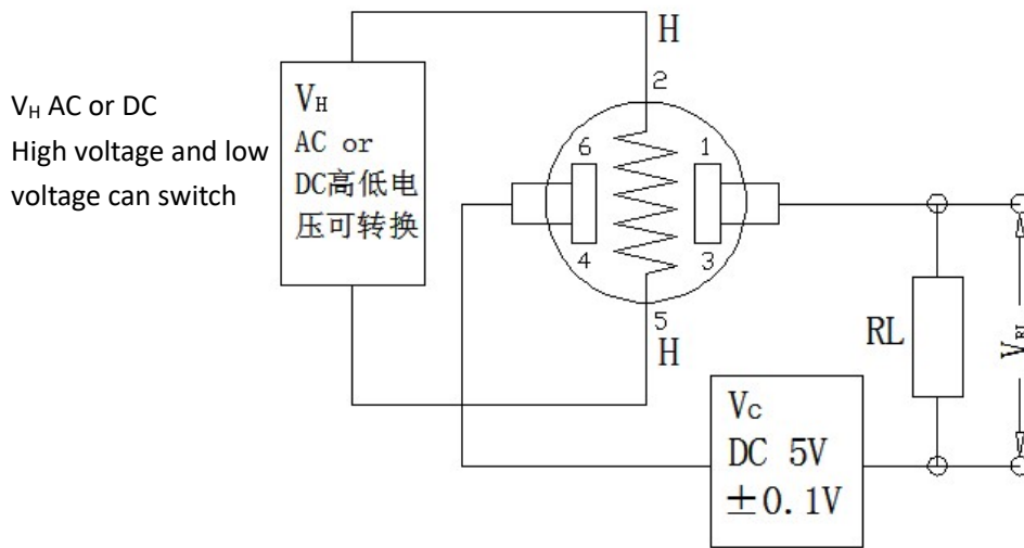
Fig2. MQ-9B Test Circuit
