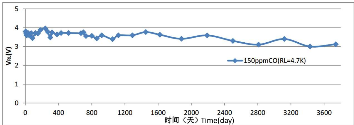
Fig7.long-term Stability
