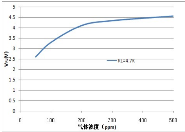
Fig5.Sensivity Curve
